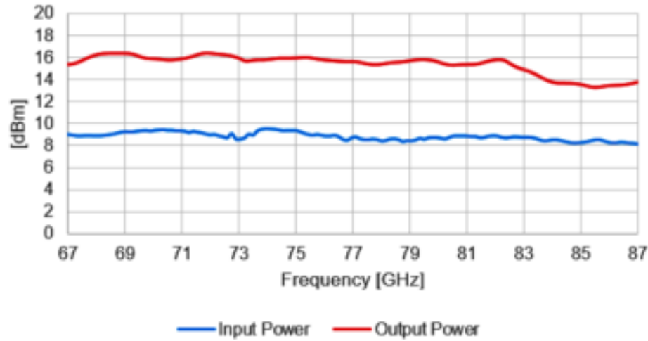
Saturated Output Power S/N 100002
